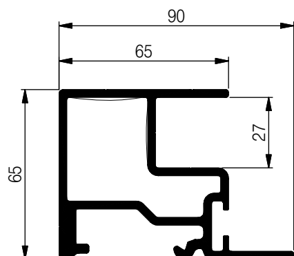
Rungen Slider Montant Slider Pillar Slider 56 000 L = 4950 3.015 kg/m
