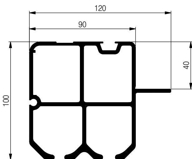
Laufschiene Slider Rail Slider Rails profile Slider 56 020 L = 7000 56 020-1 L = 4500 4.964 kg/m
