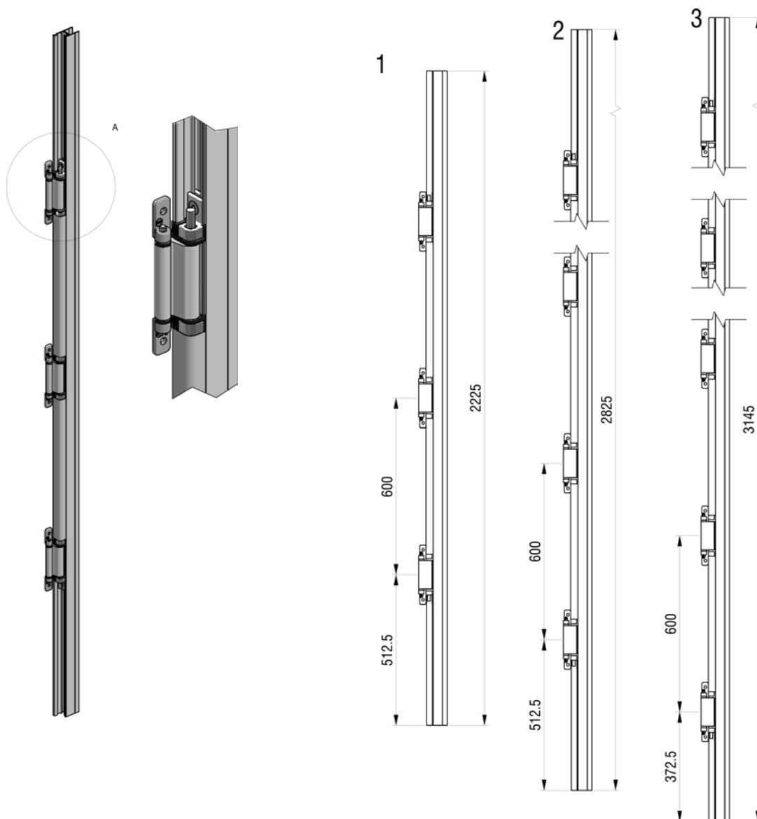
Scharnier Challenge
